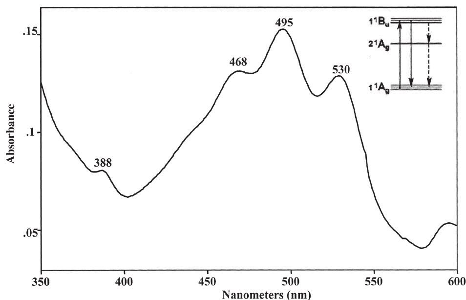
FIG. 3. The electronic absorption spectrum of acetone-soluble extract of Hbt. salinarum NRC-1 cells. Absorptions occur as broad bands in the blue/green spectral range with \lambda_{\text{max}} at 468, 495, and 530 nm characteristic for an absorption spectrum for bacterioruberin. The insert shows an energy level diagram for carotenoids.
