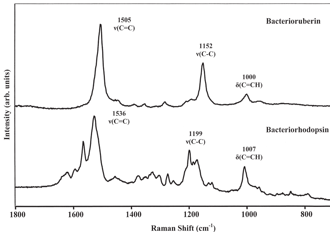
FIG. 6. Stacked resonance Raman spectra of bacterioruberlin and bacteriorhodopsin acquired from Hbt. salinarum NRC-1. Collection parameters for both spectra are 514.5 nm excitation, 10 s exposure, 5 accumulations, and 1.2 mW laser power at the sample on an InVia Reflex Renishaw Raman spectrometer. RR-enhanced modes at 1505 \text{cm}^{-1} and 1152 \text{cm}^{-1} are due to in-phase C=C ( \nu_1 ) and C-C stretching ( \nu_2 ) vibrations of the polyene chain in carotenoids, and in-plane rocking modes of CH 3 groups attached to the polyene chain coupled with C-C bonds occur in the 1000 \text{cm}^{-1} region and can be observed for bacterioruberlin. While four vibrational modes can be observed for bacteriorhodopsin: the C=C stretches (1600–1500 \text{cm}^{-1} ), the CCH in-plane rocks (1400–1250 \text{cm}^{-1} ), the C-C stretches (1250–1100 \text{cm}^{-1} ), and the hydrogen out-of-plane wags (1000–700 \text{cm}^{-1} ).
