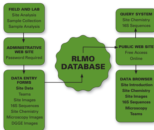
↑ Figure 2. RLMO Database Structure. This flow chart schematically illustrates the conceptual design of the database, following the process from field collection and analysis through data tables for administrative entry and public viewing.
