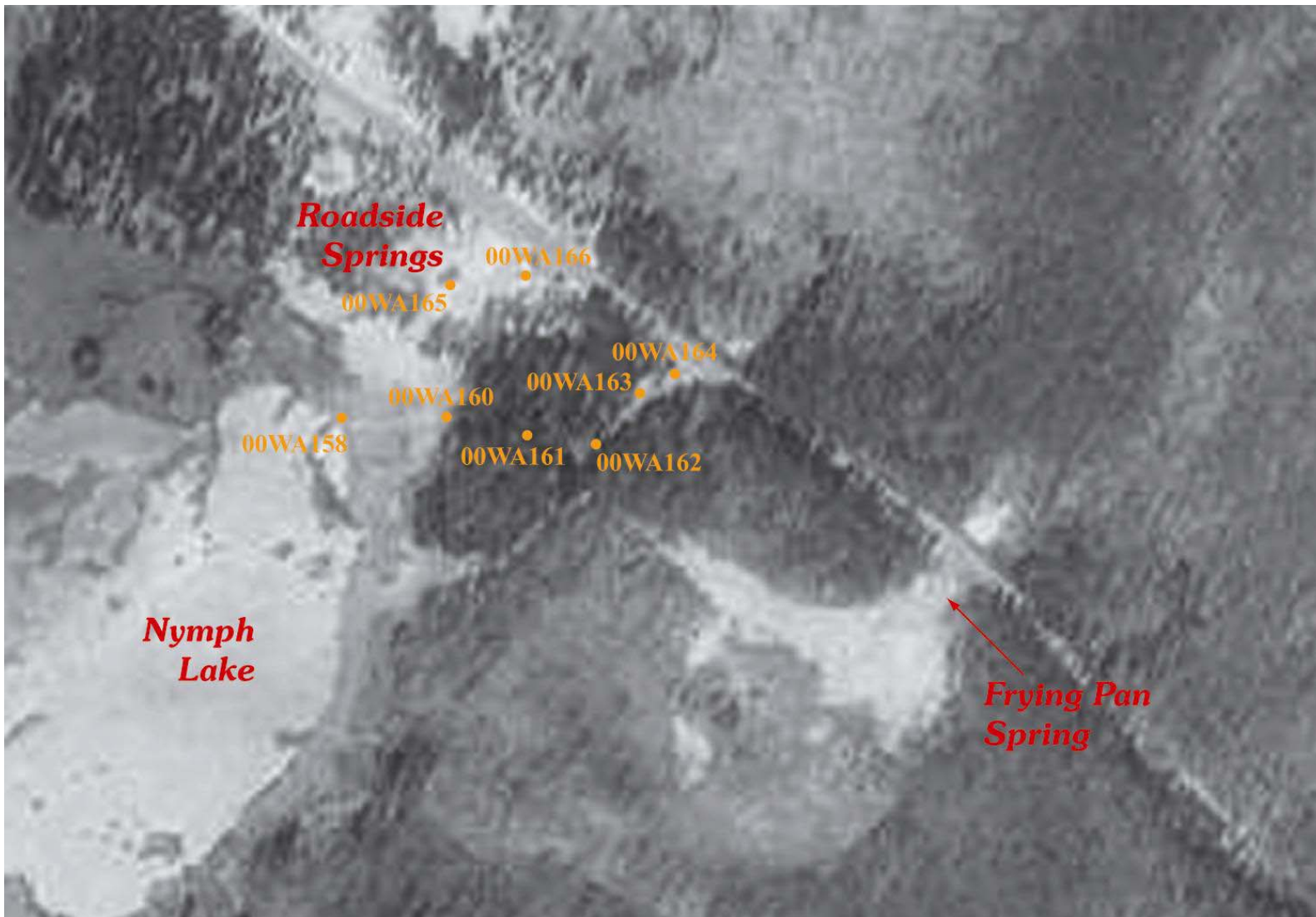
Figure 6. Sampling locations for Nymph Creek, two vents of Nymph Creek Springs, and two of the Roadside Springs near Nymph Lake, Yellowstone Park, Wyo.
