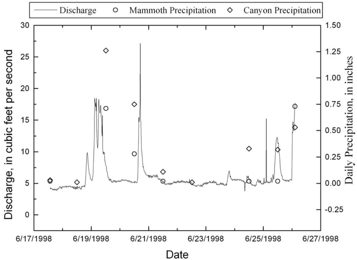
Figure 12. Local daily precipitation and Tantalus Creek discharge for June 17 to 27, 1998
