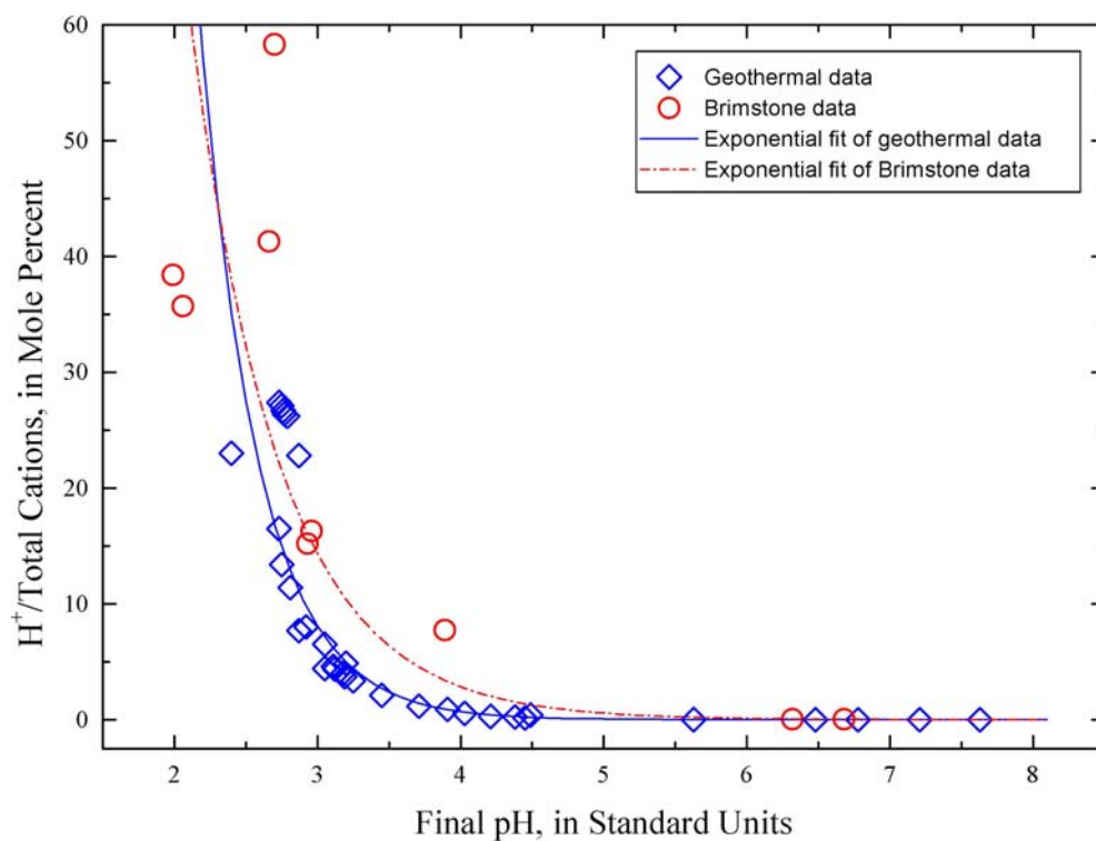
Figure 14. Mole percentage of H^+ comprising total cations as a function of final pH
