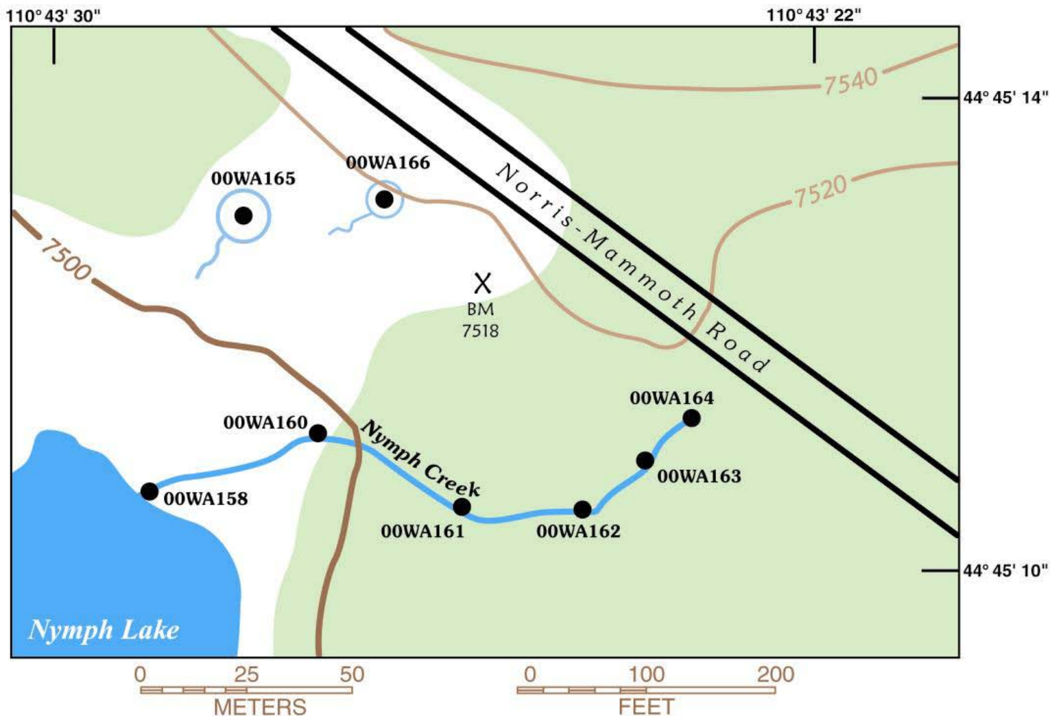
Figure 7. Sampling locations for Nymph Creek, two vents of Nymph Creek Springs, and two of the Roadside Springs near Nymph Lake, Yellowstone Park, Wyo.
