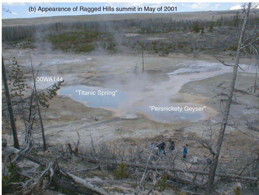
Figure 10. Photographs comparing development of thermal features at the crest of The Gap, Norris Geyser Basin
