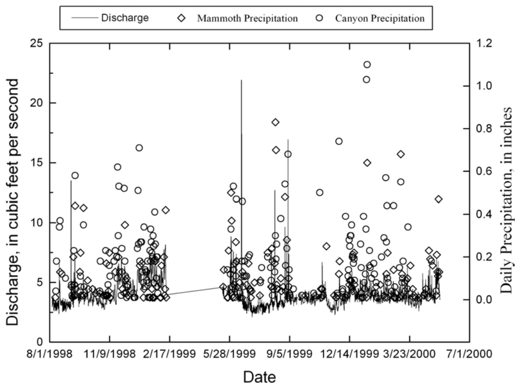
Figure 11. Local daily precipitation and Tantalus Creek discharge for August 5, 1998 to May 13, 2000 (Friedman, I. A., unpublished data)
