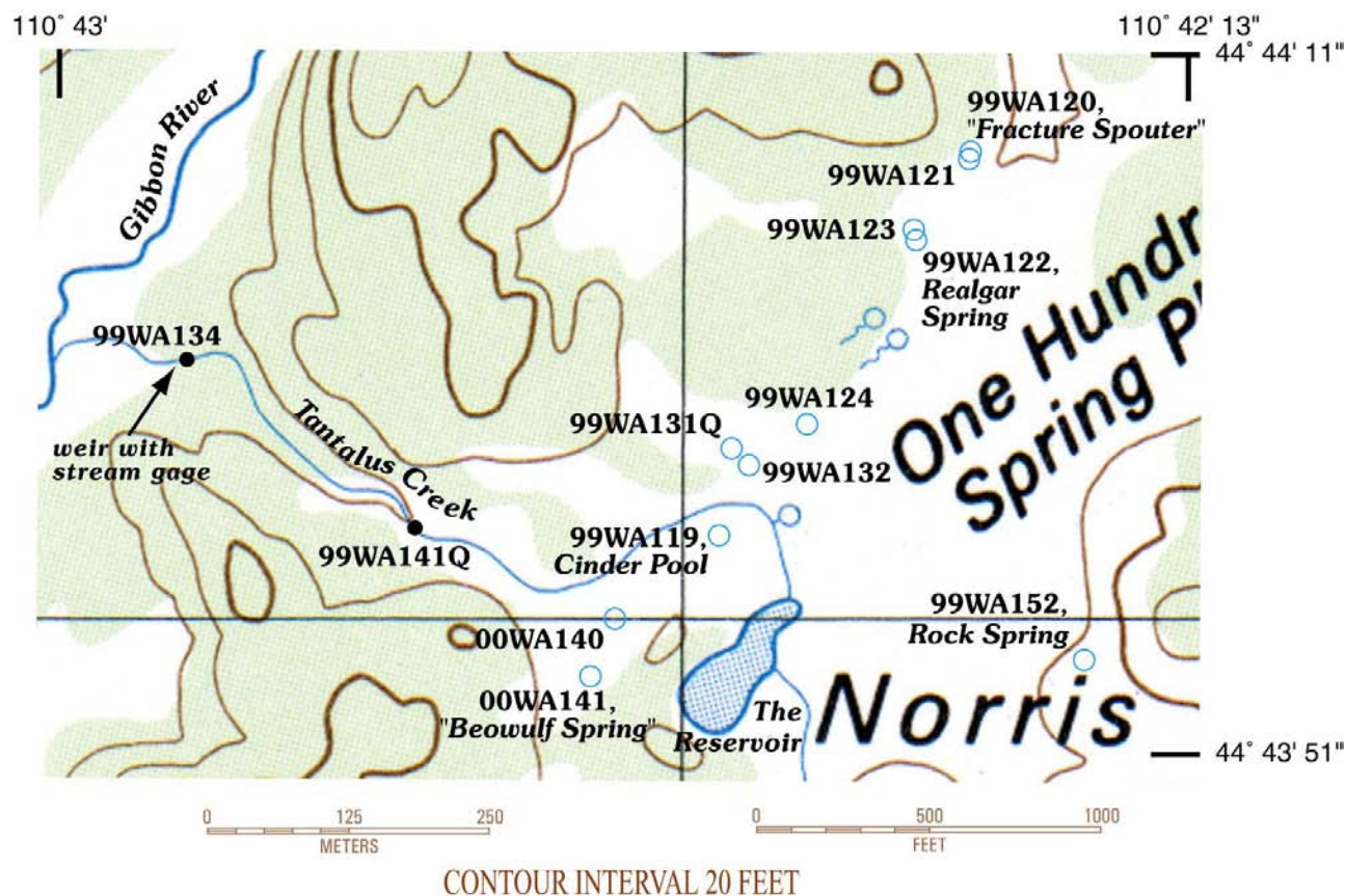
Figure 3. Sampling locations for hot springs and two surface water samples in the One Hundred Spring Plain area of Norris Geyser Basin, Yellowstone National Park, Wyo.
