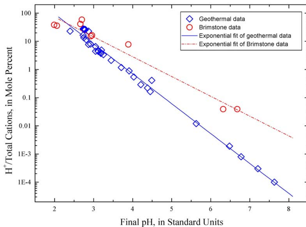
Figure 15. Semi-log plot of mole percentage of H^+ comprising total cations as a function of final pH
