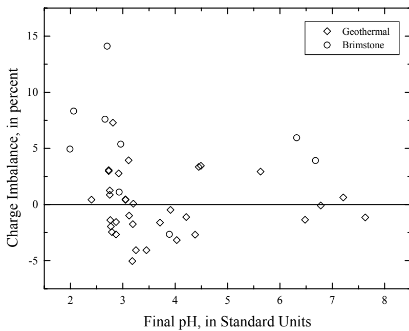
Figure 16. Speciated solution charge imbalance as a function of final pH
