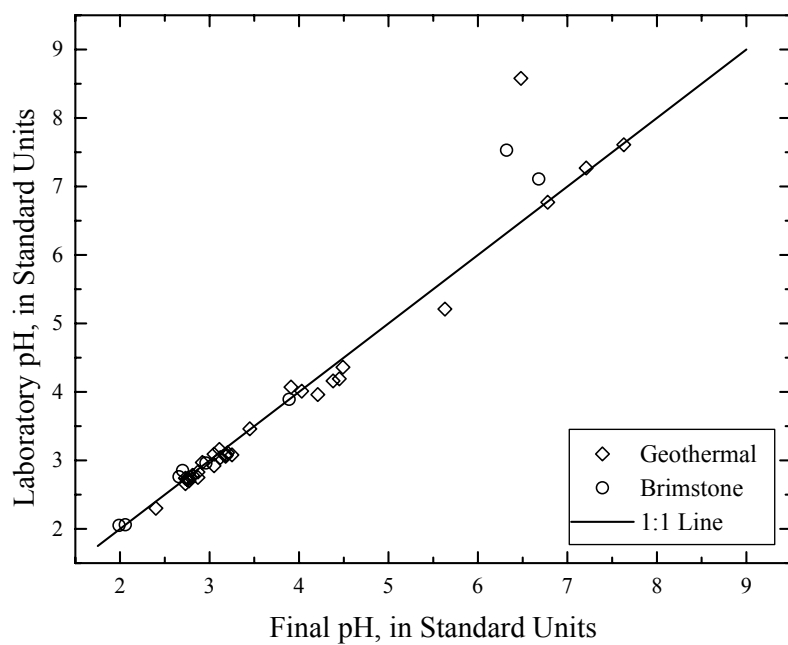
Figure 17. Laboratory pH as a function of final pH
