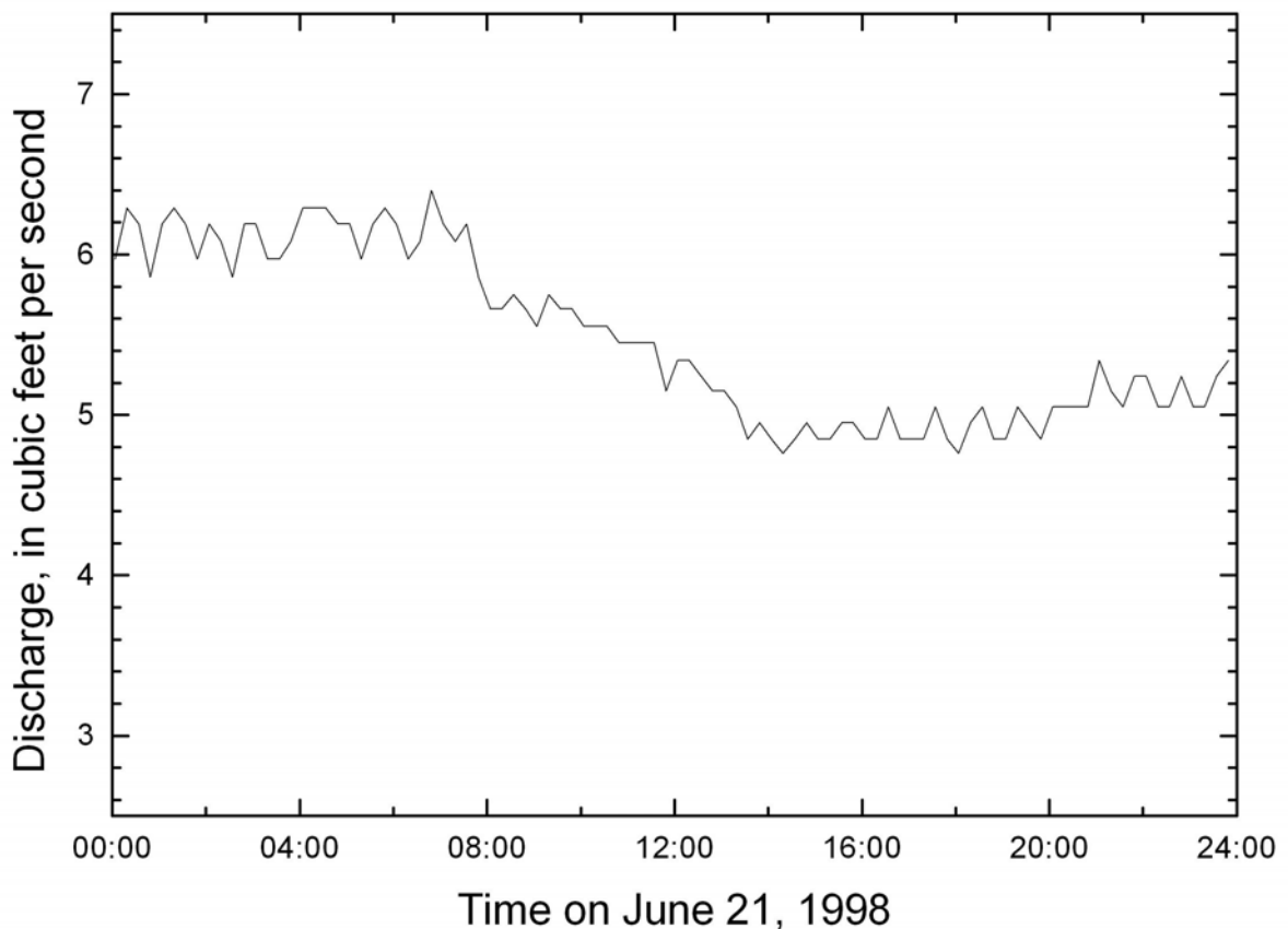
Figure 13. Tantalus Creek discharge for a 1-day period. Total precipitation for the day was 0.02 in at Mammoth and 0.11 in at Canyon Village
