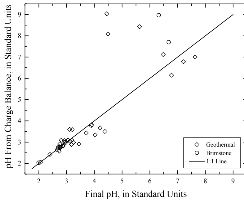
Figure 19. Charge balance pH as a function of final pH
