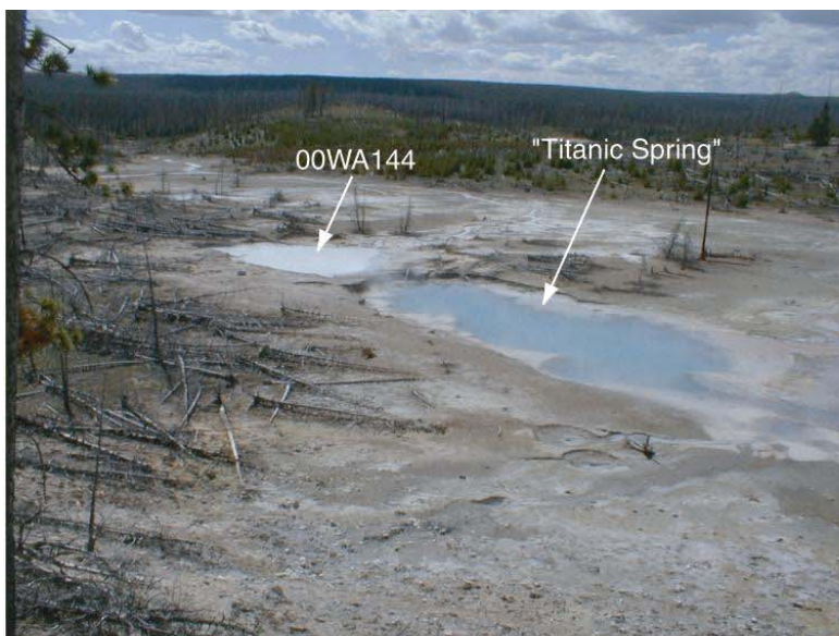
Ragged Hills summit showing 00WA144 and "Titanic Spring"
