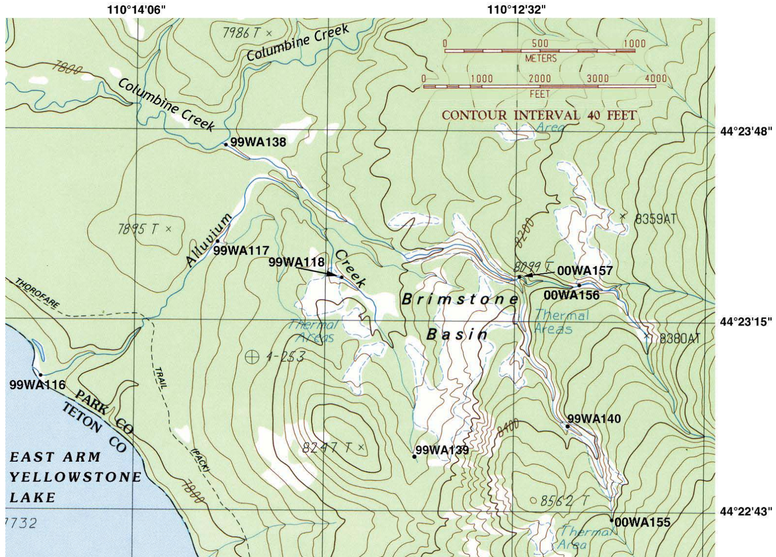
Figure 8. Sampling sites for Alluvium and Columbine Creeks and their tributaries, Yellowstone National Park, Wyo.
