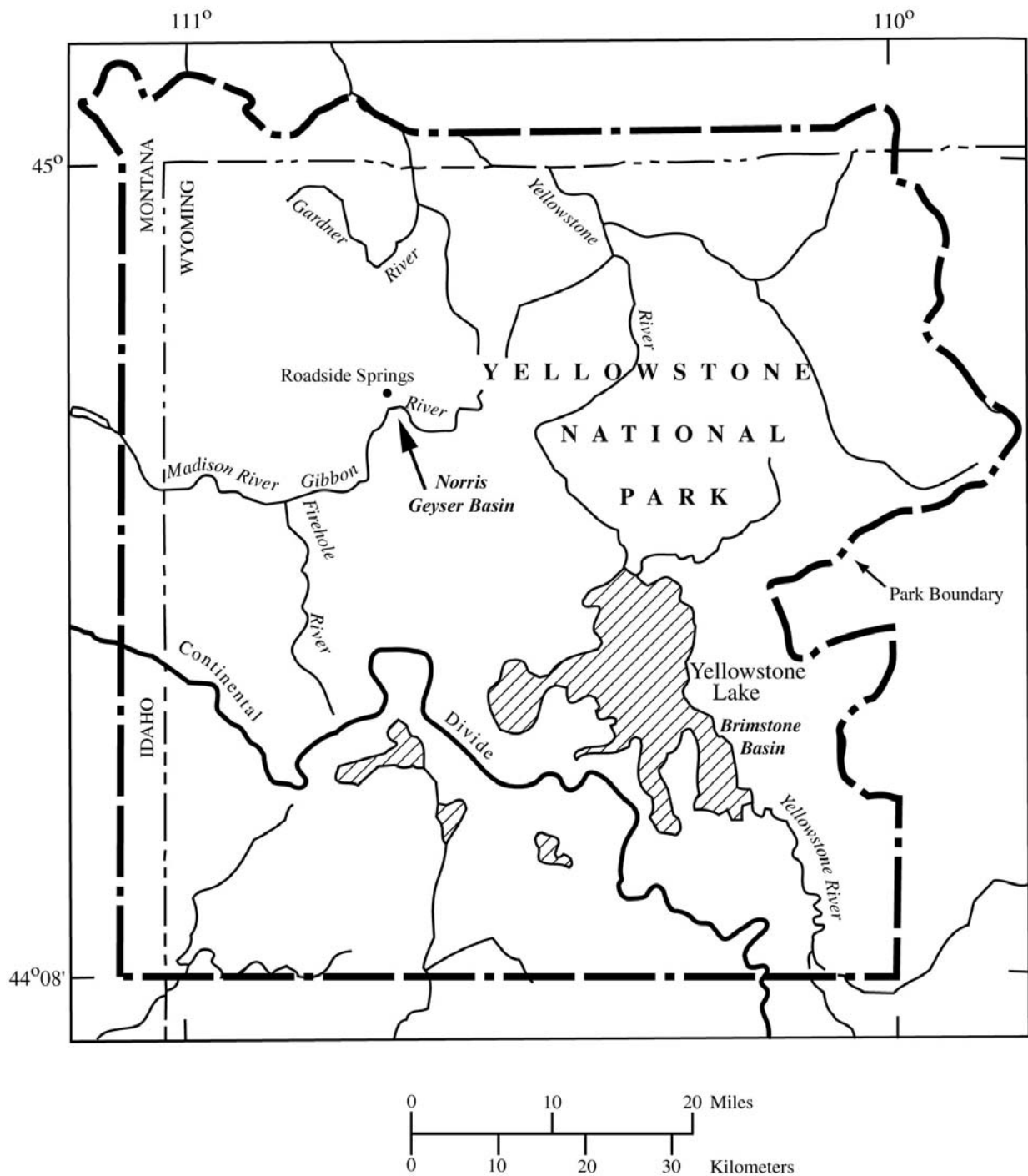
Figure 1. Location of sampling areas in Yellowstone National Park, Wyo.
