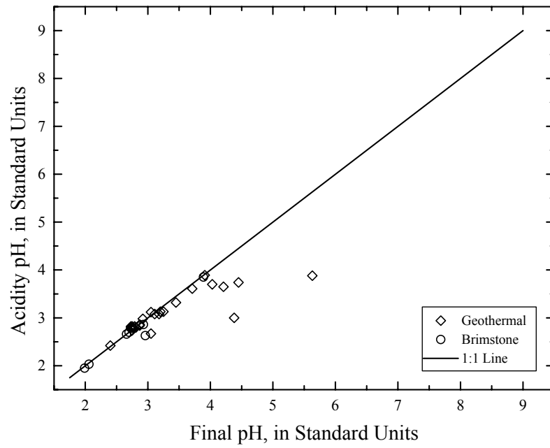
Figure 18. Acidity pH as a function of final pH
